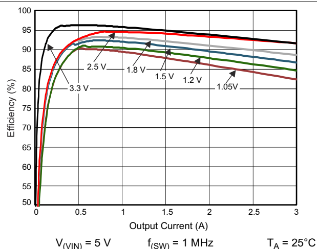
图 8-5. Efficiency vs Load Current
