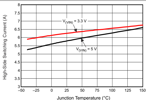
图 6-3. High-Side Current Limit vs Temperature
